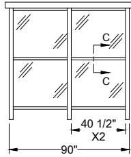
ELEVATION D
