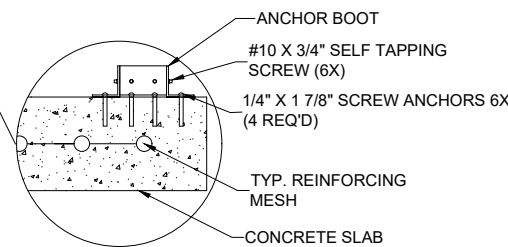
ANCHORING DETAIL
