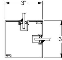
VIEW B-B
